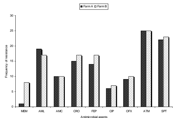
Figure 1 Frequency of multiresistance in E. coli isolates against antimicrobials.
