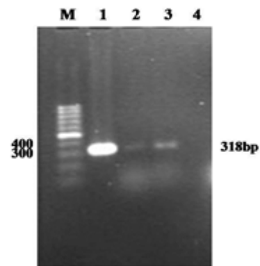
Figure 1 PCR products from positive L. intracellularis fecal samples were amplified 318 bp fragments. (Lane M was 100 bp DNA ladder marker, Lane 1 was positive control, Lane 2 and 3 were positive L. intracellularis and Lane 4 was negative control)
